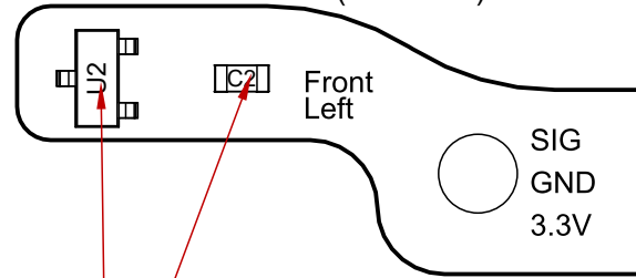
View from Bottom side (Scale 4:1)
