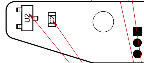
View from Bottom side (Scale 4:1)
